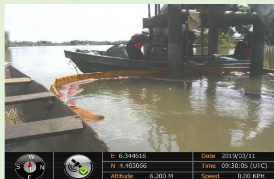
Plate 10: Deployment of hand pulling canoe for recovery activities
